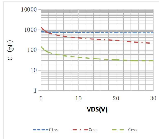
Fig.2 Capacitance Characteristics
